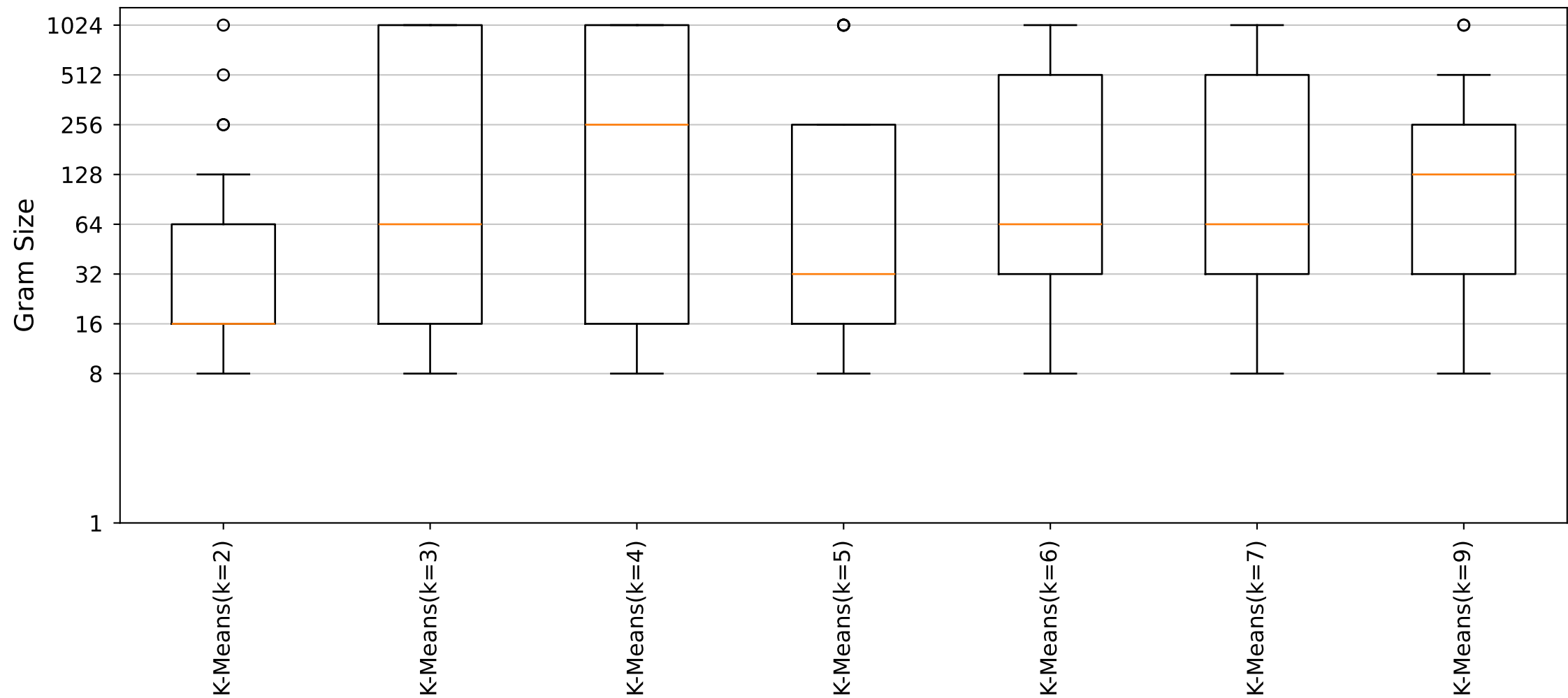
YARA Rules Gram Size Distribution (Cluster14_Size9 dataset)
